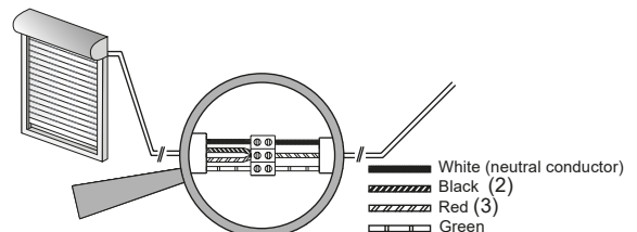
Fig. 7 Radio connection (transmitter operation)
