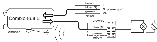
Connection diagram with/without ballast
