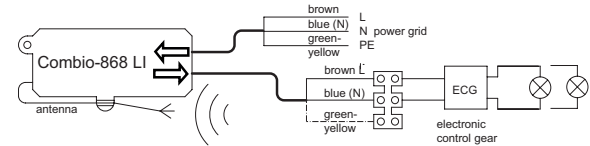
Connection diagram with/without ballast
