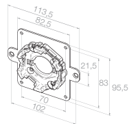
230040101 Motor bearing for SKS torque limitation Max. 50 Nm
