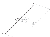
16 103.1901 Height: 2.0 mm Stud spacing: 22.0 mm (Motor centre with 2 holes)
