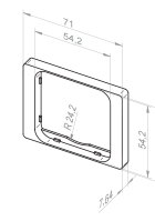
14 303.1601 White, suitable for: – Berker Arsys
