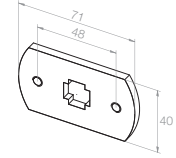
13 301.7001 Wall bracket, flat, Pitch circle of 48 mm
