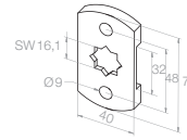
13 110.5601 Spacer plate for 13 103.3901 (cannot be used as bearing)
