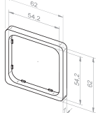
14 303.1101 Alpine white, suitable for: – Gira surface (before 2007)
