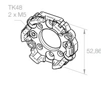
230030401 Pitch circle of 48 mm with 2 x M5 nuts, pitch circle of 60 mm
