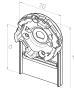
23 615.8401 For built-in roller shutters, size 165 mm, d = 78.2 - 79.7 mm, up to max. 30 Nm
