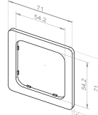
14 303.1401 White, suitable for: – Gira Standard – Gira surface (after 2007)
