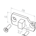
230990001 With 10 x 6.5 mm bolt (11 mm high) incl. fixing screws
