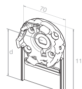
236159401 For built-in roller shutters, size 165 mm, d = 78.2 - 79.7 mm, up to max. 30 Nm
