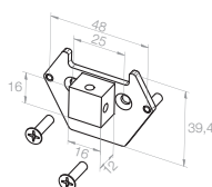
233742101 16 x 16 mm, 12 mm pin
