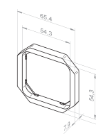
14 303.0801 White, suitable for: – Merten Octocolor
