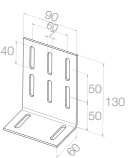
13 110.5101 130 mm high
