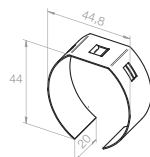
133018501 For T-spring 50 mm, octagonal shaft
