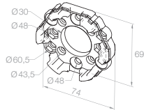
23 003.0001 Pitch circle 48/60 (aluminium)
