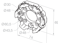
230030001 Pitch circle 48/60 (aluminium) with 4 x M6 nuts
