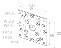
13 109.2902 Base plate with 48/60/90 mm pitch circle (without motor bearing and screws)
