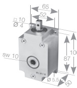
23 030.0001 Angle drive
