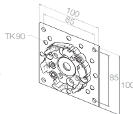
236159901 Base plate with motor bearing, e.g. for VEKA variant elements
