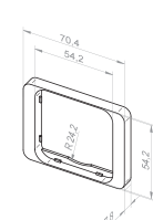
14 303.0901 Alpine white, suitable for: – Busch-Jaeger alpha-nea
