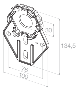
23 004.0001 Universal motor bearing (plastic) Torque limitation of max. 50 Nm
