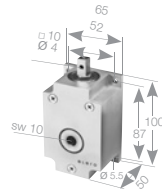
23 030.0001 Angle drive
