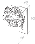
23 615.9101 Motor bearing, cranked, up to max. 50 Nm (60 mm wall distance)
