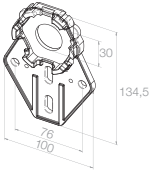
230040001 Universal motor bearing (plastic), torque limitation, max. 50 Nm
