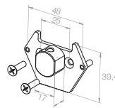
23 374.9801 Adapter plate with bolt, Ø 19.5 mm Compatible with Becker bearing
