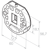
23 986.0001 Wall anchor, latching, Pitch circle of 48 mm
