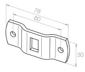
13 106.1701 Wall bracket, cranked, Pitch circle of 60 mm
