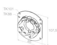
236157101 Mounting plate with plastic bearing up to max. 30 Nm (Thyssen, Schüco, Veka, Home)
