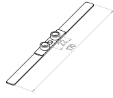
161016101 Height: 2.0 mm Hole spacing: 22.0 mm (motor centre)
