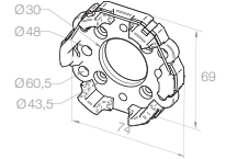
23 003.0301 Pitch circle 48/60 with M6/M8 thread - for awnings -
