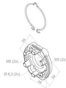
23 617.6001 Awning bearing with safety clip (small eyelet)
