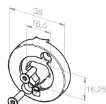
220420101 Without leaf, white, comple- te, incl. mounting accesso- ries with long screws for use with following metal adapter plates
