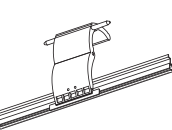
133018901 2-membered
