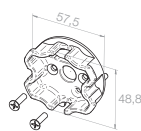
233749401 SH adapter (up to 50 Nm) Compatible with Somfy and Selve star head bearings
