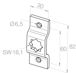
13 106.3501 16 x 16 mm, Pitch circle of 60 mm, cranked
