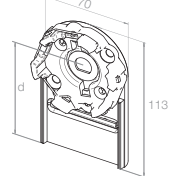
23 615.9401 For built-in roller shutters, size 165 mm, d = 78.2 - 79.7 mm, up to max. 30 Nm
