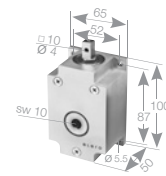
23 030.0001 Angle drive
