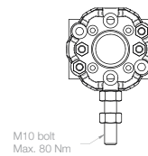
236153501 Special bolt bearing with height adjustment with M10 bolt, max 80 Nm
