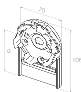
236158301 For built-in roller shutters, size 150 mm, d = 70.7 mm, up to max. 30 Nm
