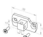
220400001 10 x 10 mm, complete, incl. accessories
